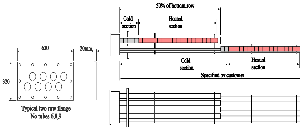
Horizontal Tank Immersion Heater
