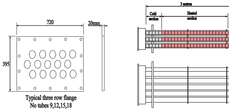
Vertical Tank Immersion Heater
