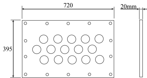
Typical three row flange No tubes 9,12,15,18
