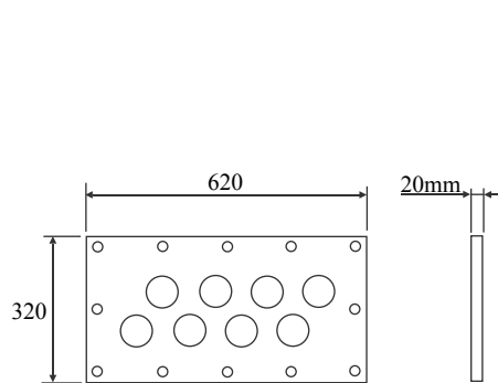
Typical two row flange No tubes 6,8,9
